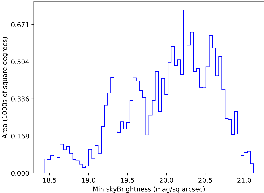
roll_pause_mjdp270_v3.4_10yrs WFD g band: Min skyBrightness
