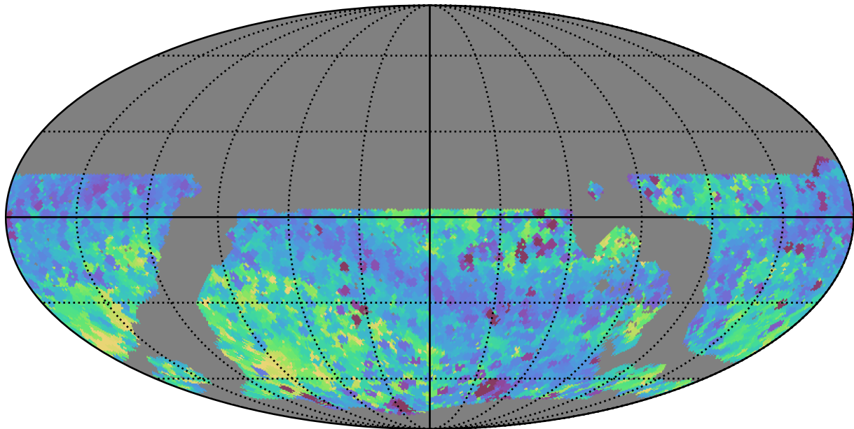
roll_pause_mjdp270_v3.4_10yrs WFD all bands: Min skyBrightness
