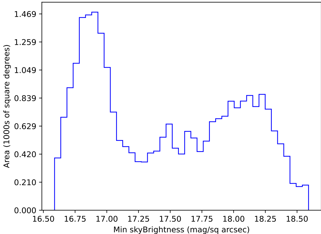
roll_pause_mjdp270_v3.4_10yrs All sky z band: Min skyBrightness
