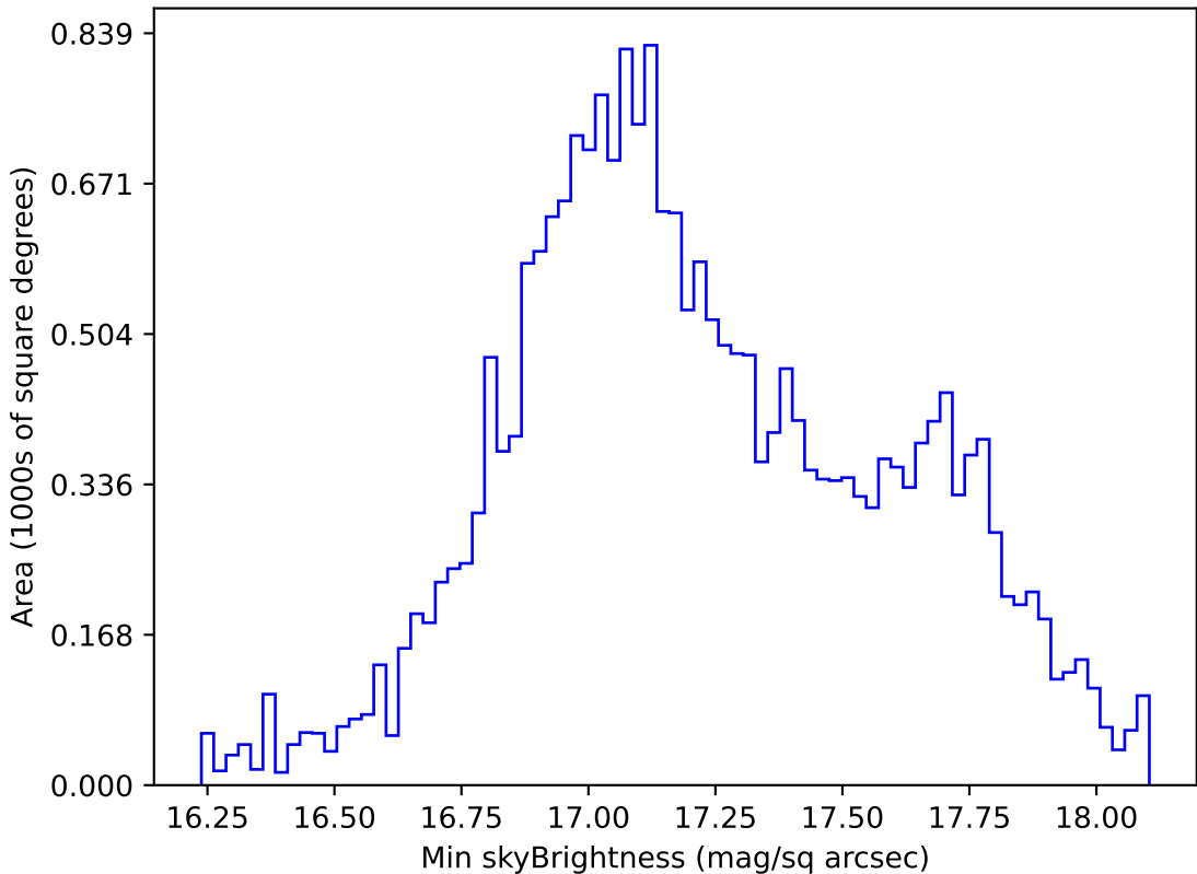
roll_pause_mjdp270_v3.4_10yrs All sky y band: Min skyBrightness
