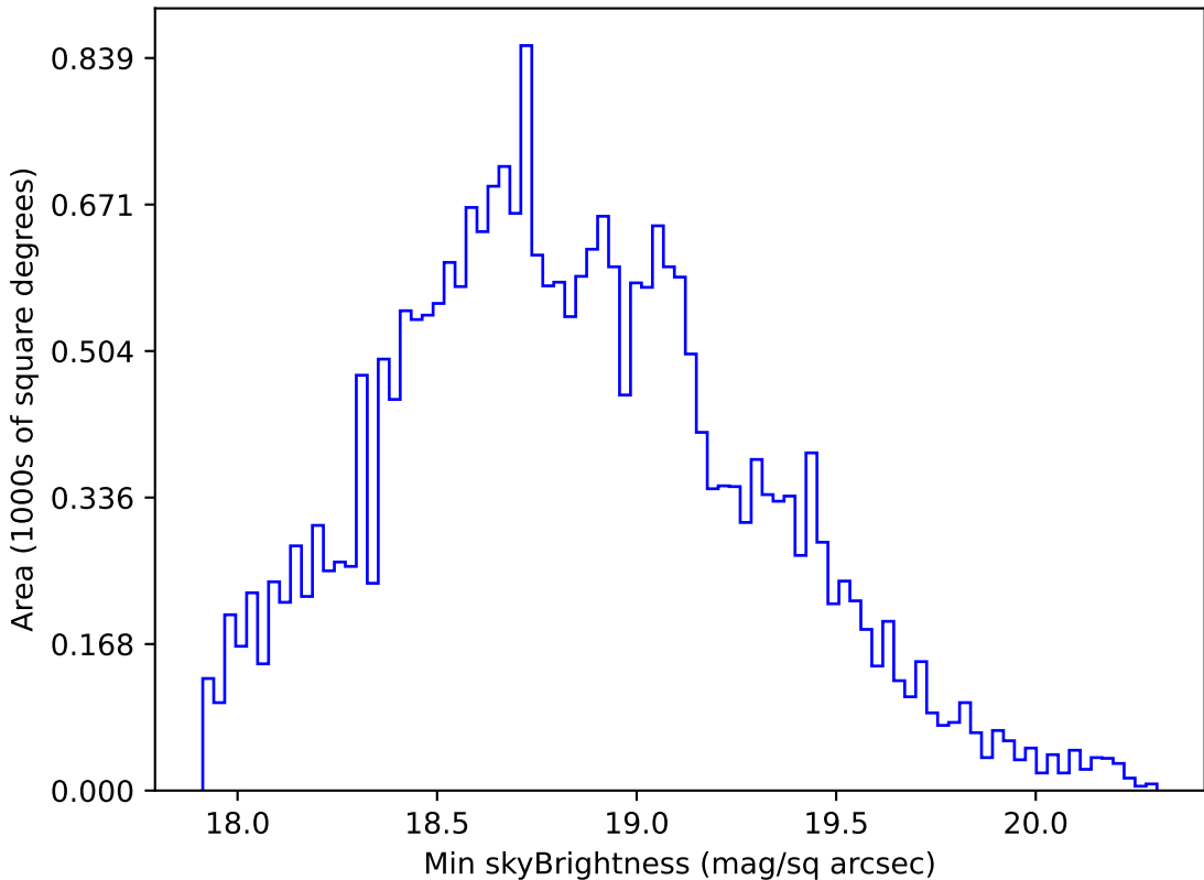
roll_pause_mjdp270_v3.4_10yrs All sky r band: Min skyBrightness
