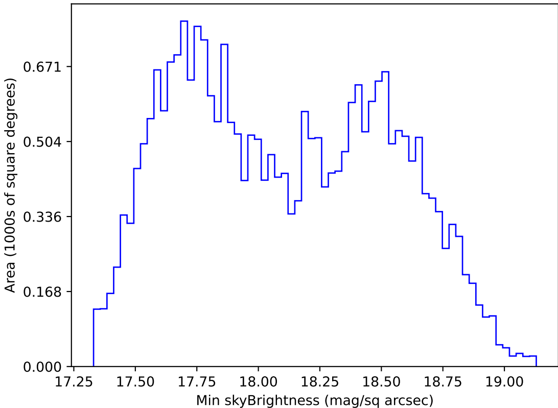
roll_pause_mjdp270_v3.4_10yrs All sky i band: Min skyBrightness
