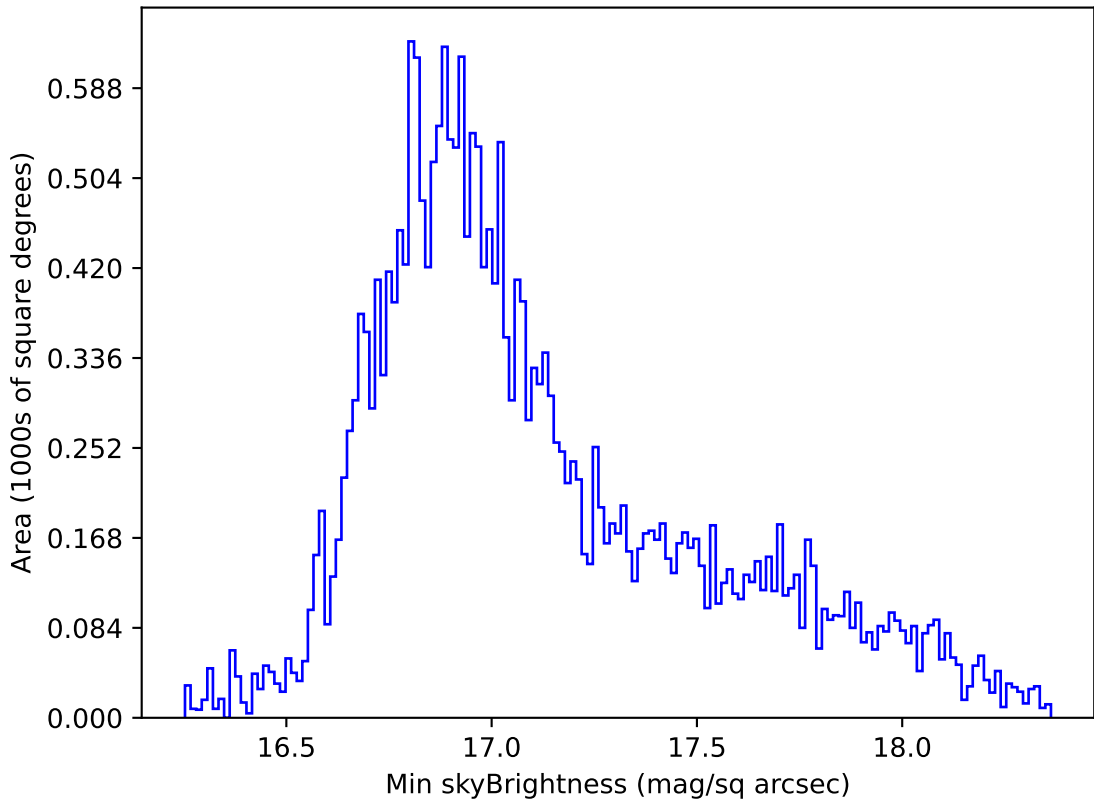
roll_pause_mjdp270_v3.4_10yrs All sky all bands: Min skyBrightness
