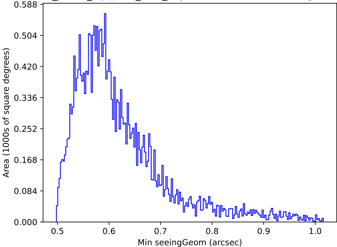
roll_pause_mjdp270_v3.4_10yrs Yr 1 z band: Min seeingGeom
