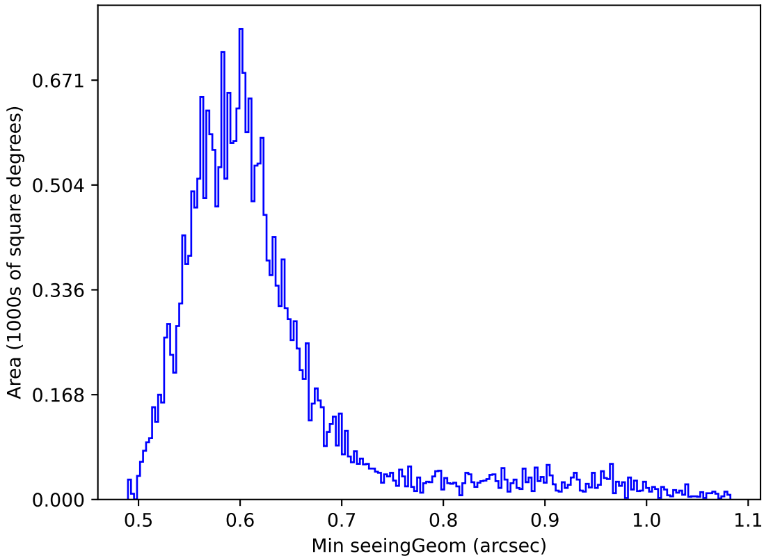
roll_pause_mjdp270_v3.4_10yrs Yr 1 r band: Min seeingGeom
