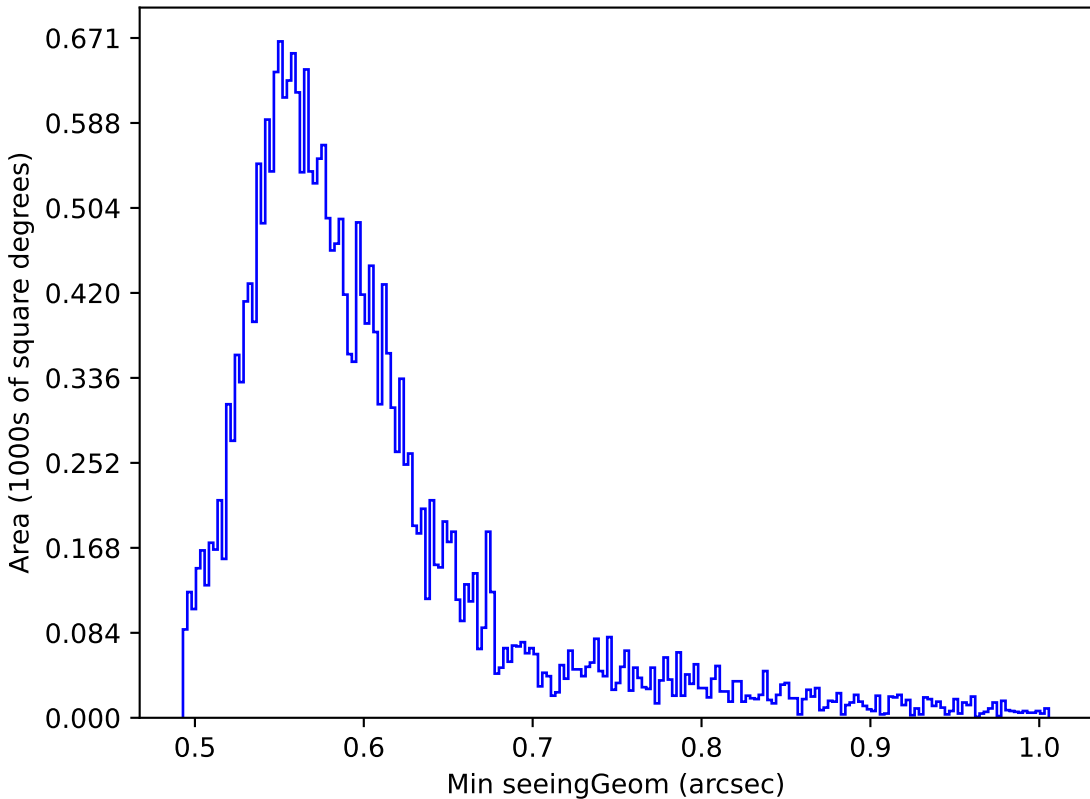
roll_pause_mjdp270_v3.4_10yrs Yr 1 i band: Min seeingGeom
