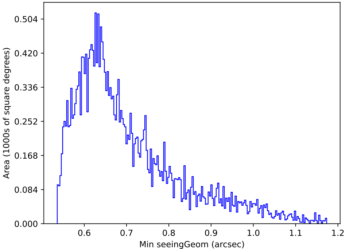
roll_pause_mjdp270_v3.4_10yrs Yr 1 g band: Min seeingGeom
