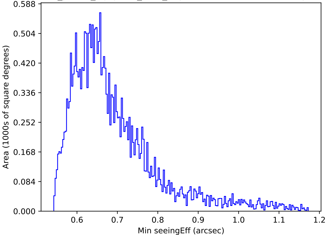
roll_pause_mjdp270_v3.4_10yrs Yr 1 z band: Min seeingEff
