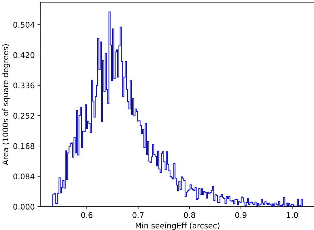
roll_pause_mjdp270_v3.4_10yrs Yr 1 y band: Min seeingEff
