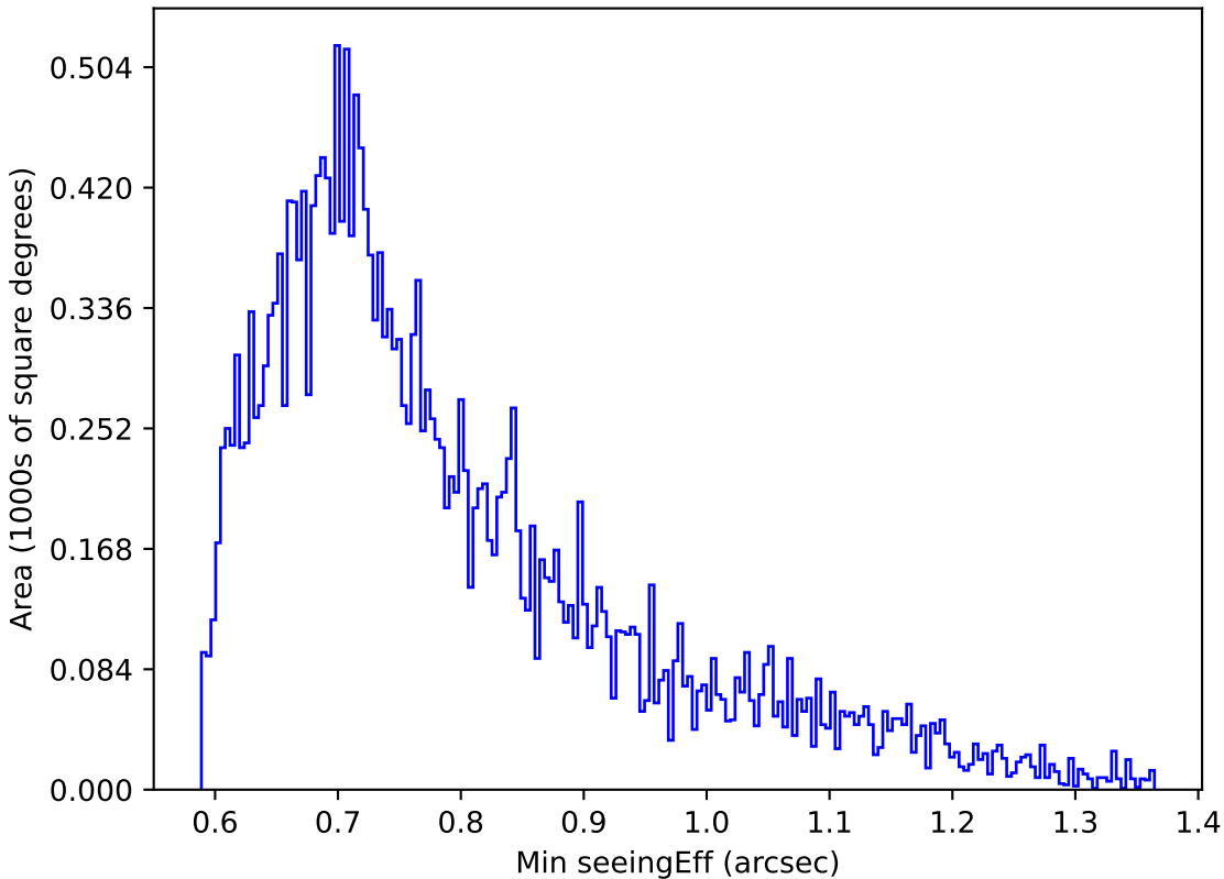
roll_pause_mjdp270_v3.4_10yrs Yr 1 g band: Min seeingEff
