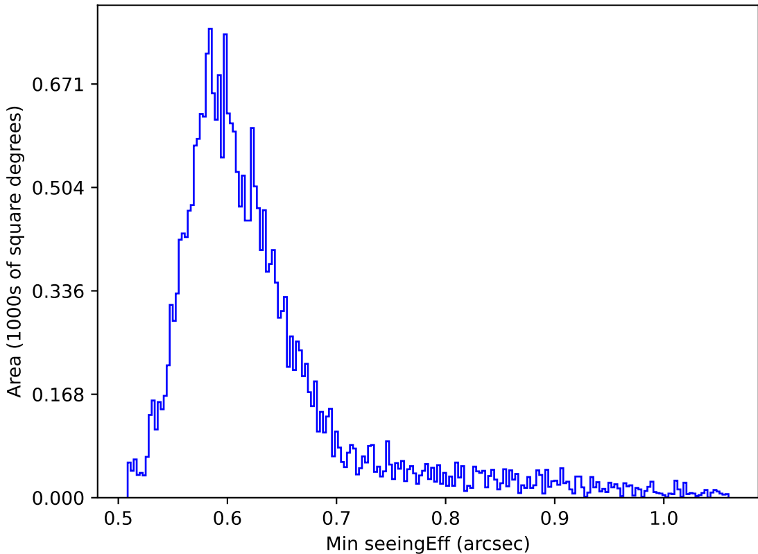
roll_pause_mjdp270_v3.4_10yrs Yr 1 all bands: Min seeingEff
