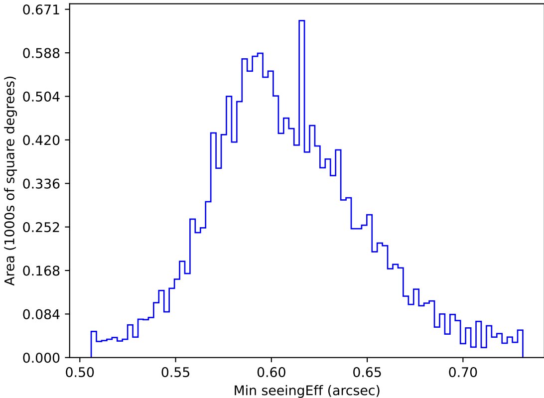
roll_pause_mjdp270_v3.4_10yrs WFD z band: Min seeingEff
