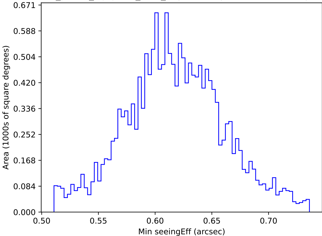
roll_pause_mjdp270_v3.4_10yrs WFD y band: Min seeingEff
