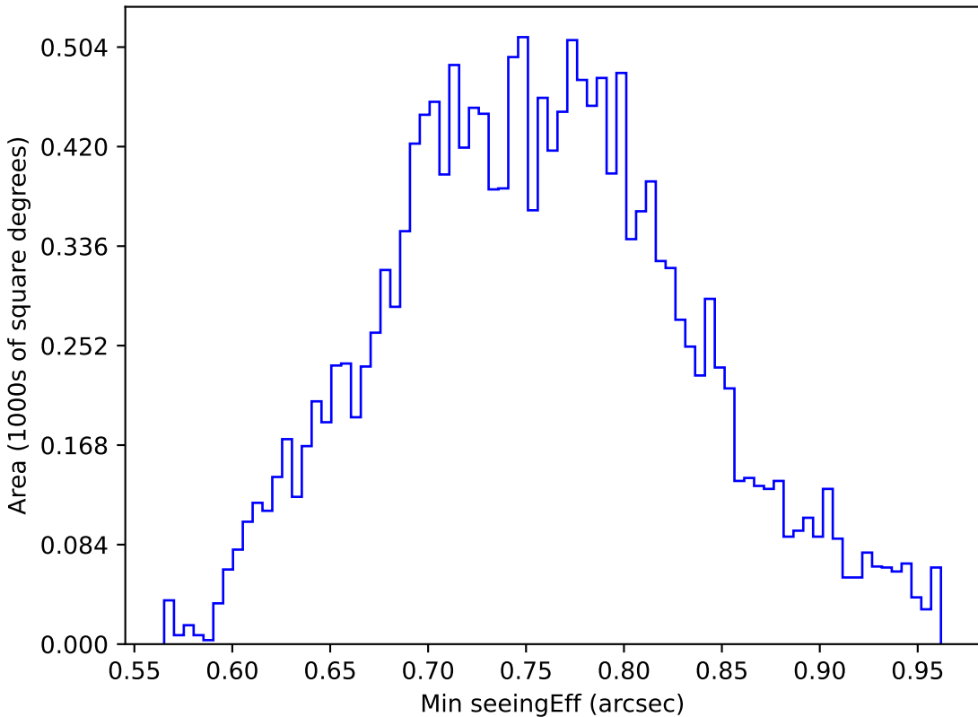
roll_pause_mjdp270_v3.4_10yrs WFD u band: Min seeingEff
