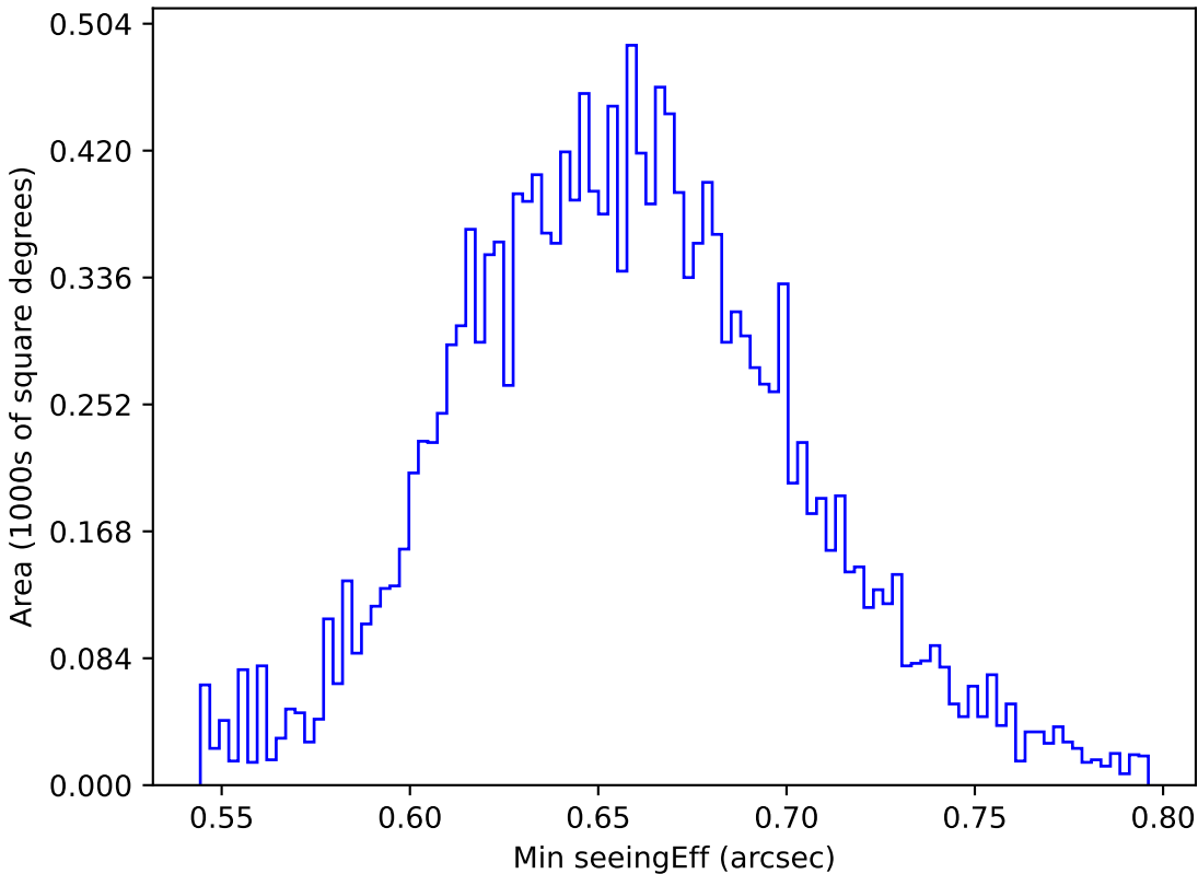
roll_pause_mjdp270_v3.4_10yrs WFD g band: Min seeingEff
