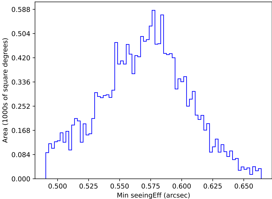
roll_pause_mjdp270_v3.4_10yrs WFD all bands: Min seeingEff
