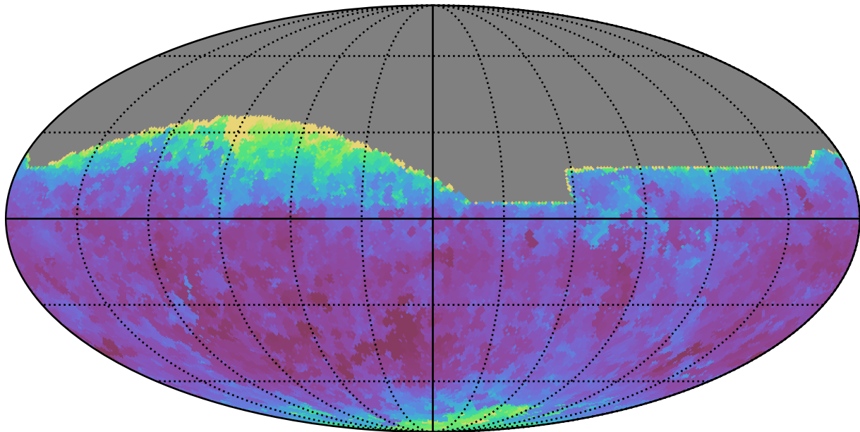
roll_pause_mjdp270_v3.4_10yrs All sky z band: Min seeingEff
