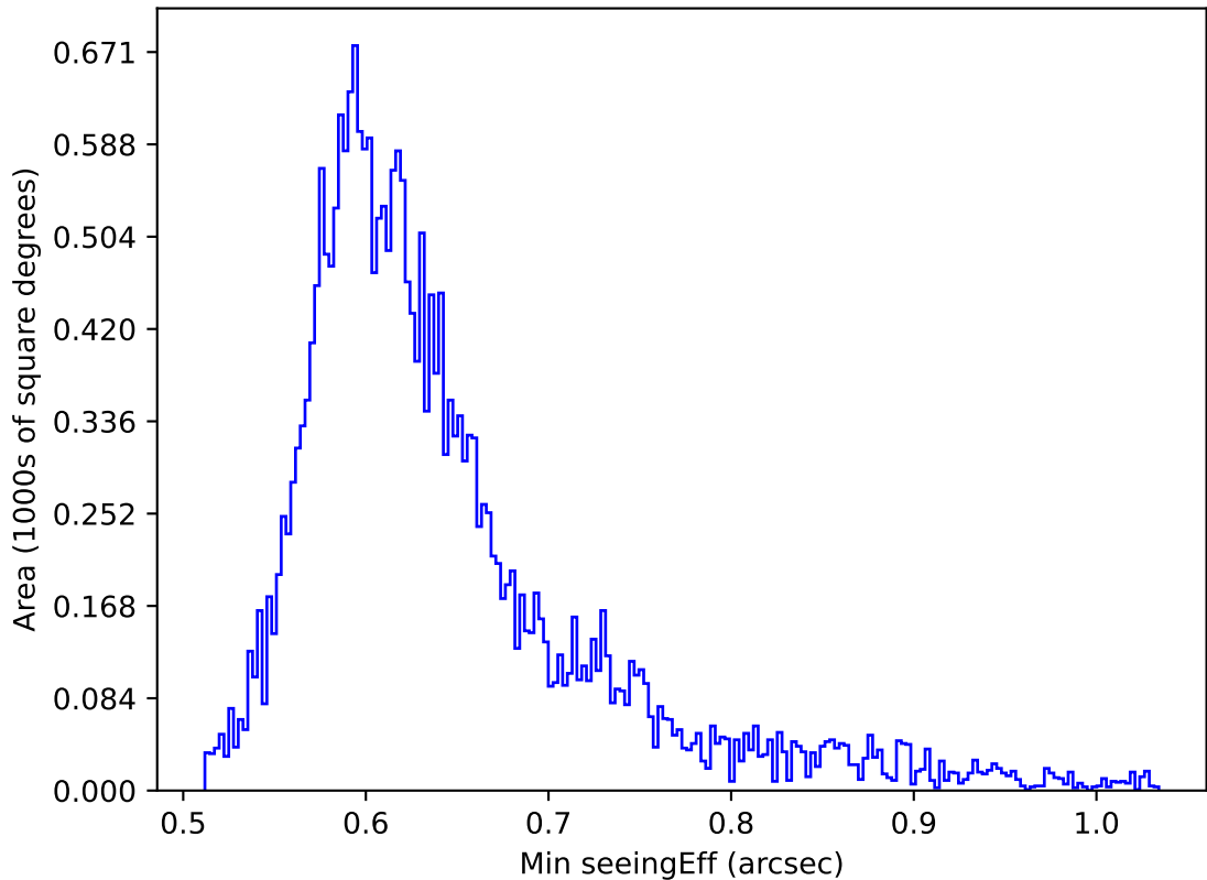
roll_pause_mjdp270_v3.4_10yrs All sky z band: Min seeingEff
