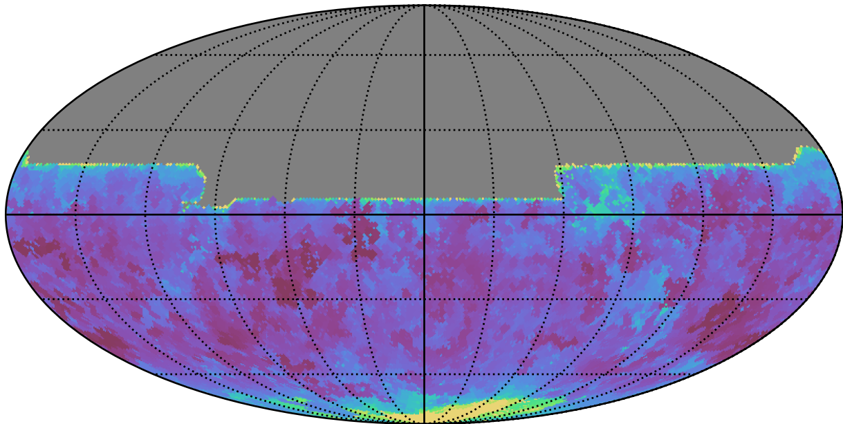
roll_pause_mjdp270_v3.4_10yrs All sky y band: Min seeingEff
