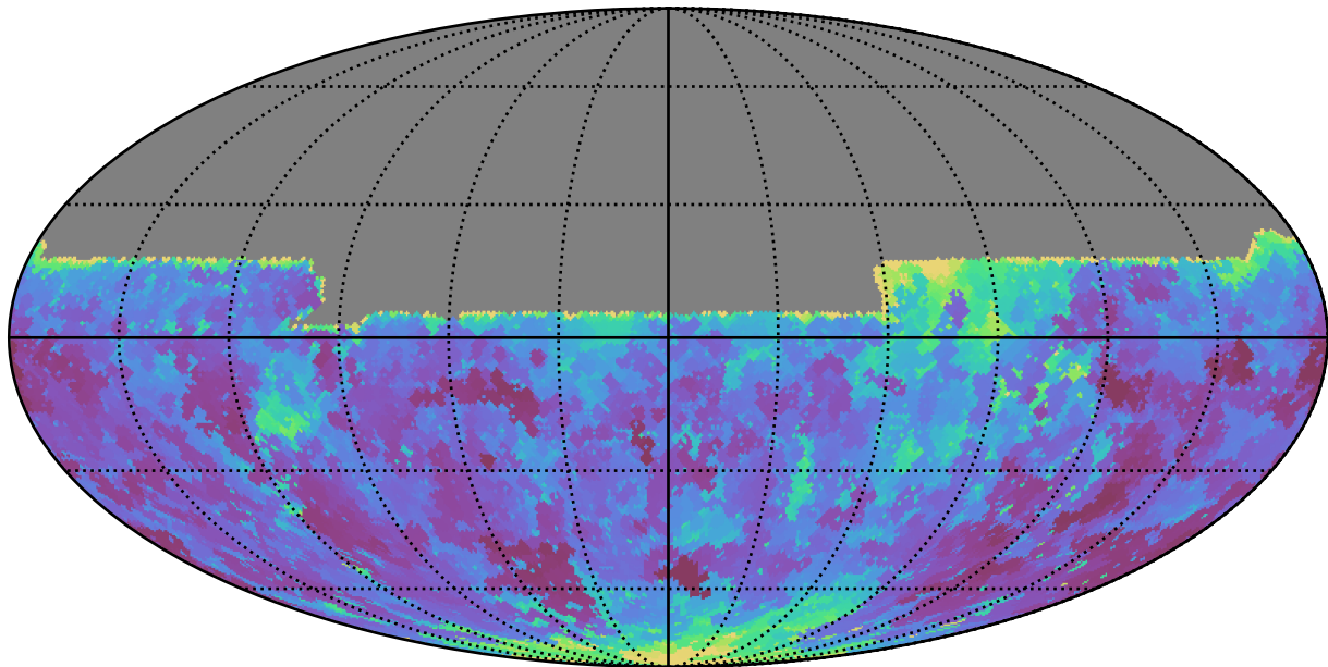
roll_pause_mjdp270_v3.4_10yrs All sky u band: Min seeingEff
