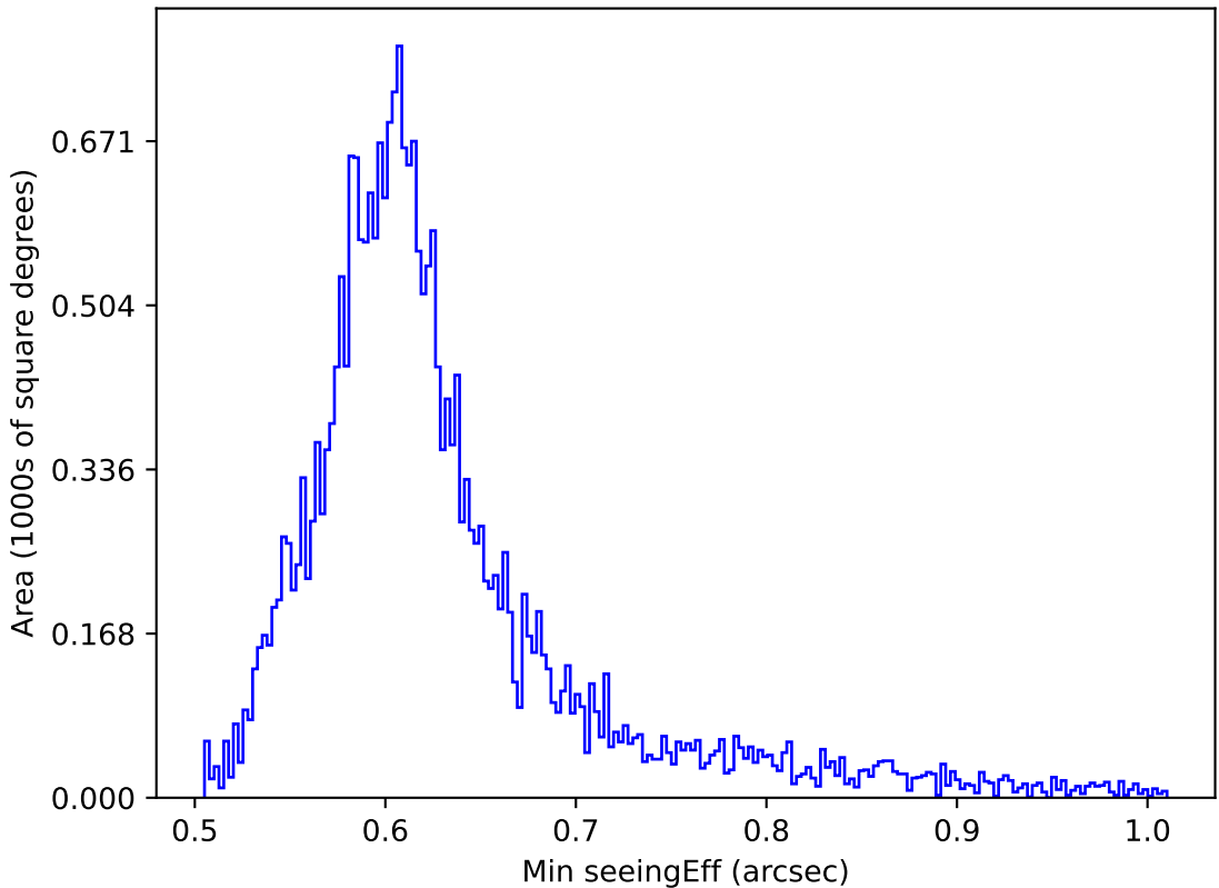
roll_pause_mjdp270_v3.4_10yrs All sky i band: Min seeingEff
