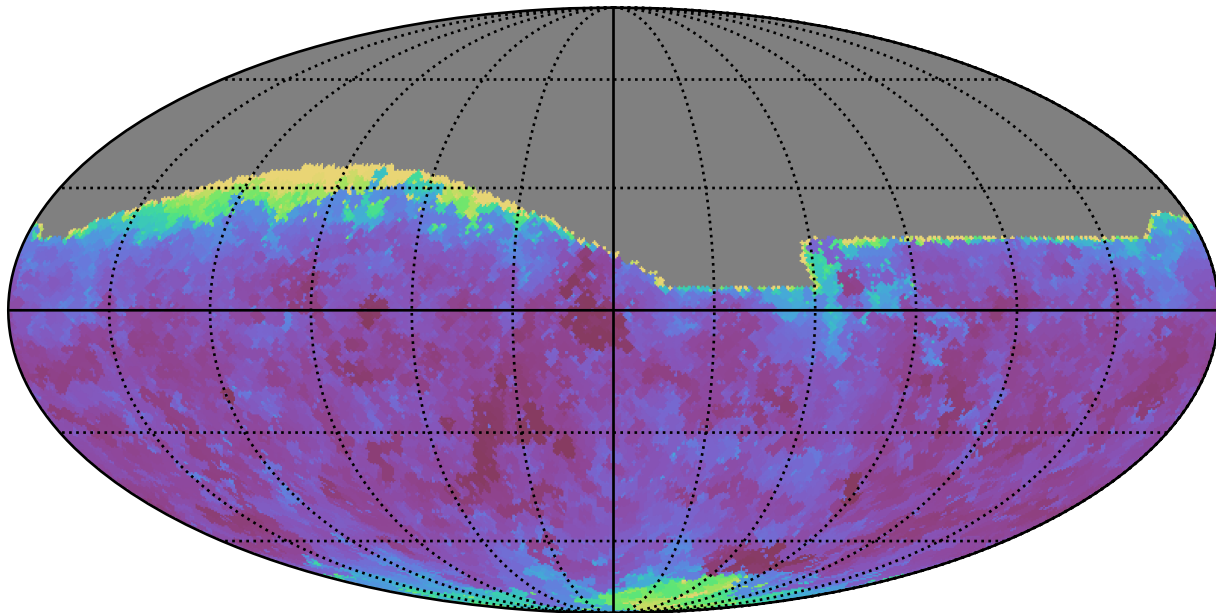
roll_pause_mjdp270_v3.4_10yrs All sky g band: Min seeingEff
