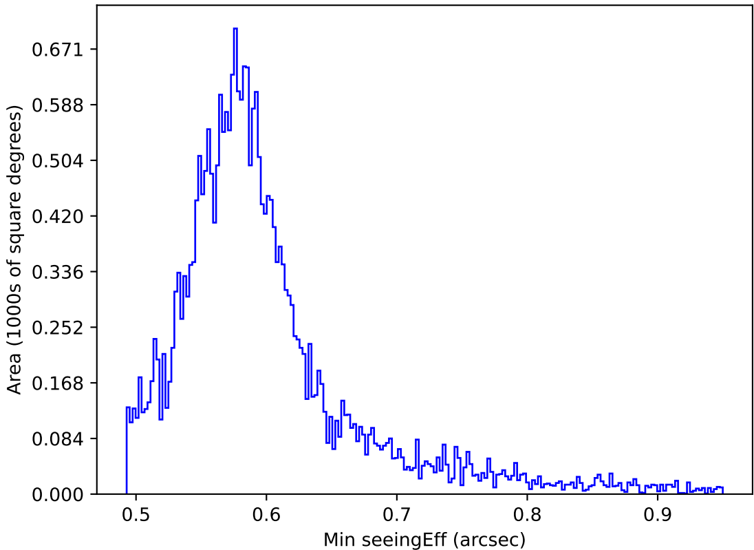
roll_pause_mjdp270_v3.4_10yrs All sky all bands: Min seeingEff
