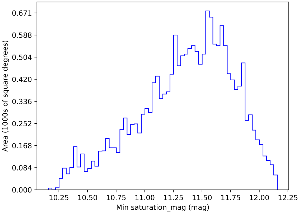
roll_pause_mjdp270_v3.4_10yrs WFD u band: Min saturation_mag
