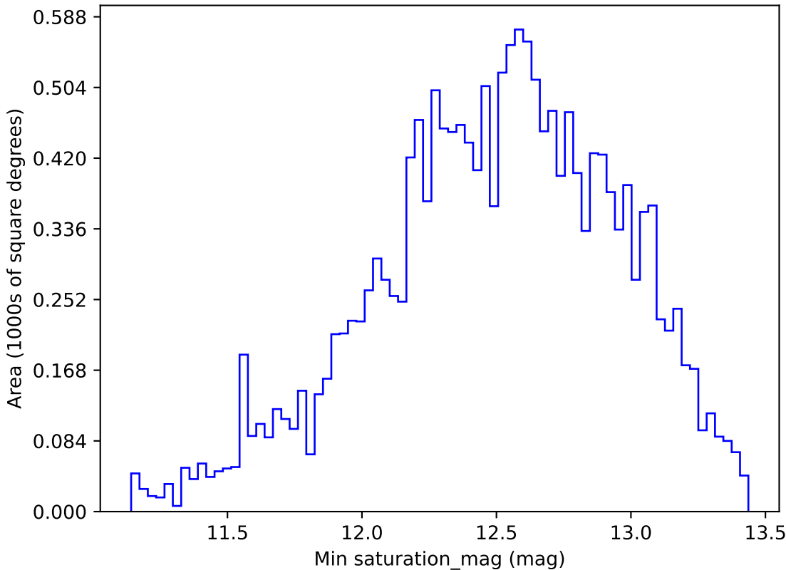
roll_pause_mjdp270_v3.4_10yrs WFD r band: Min saturation_mag
