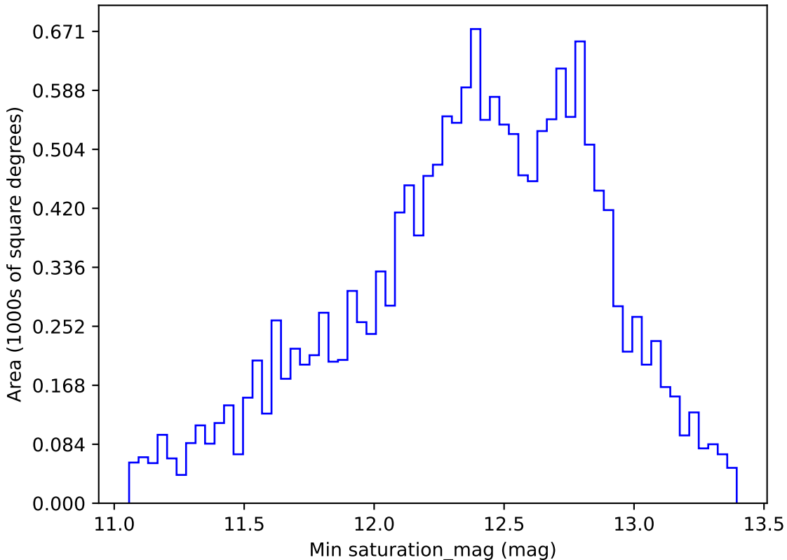
roll_pause_mjdp270_v3.4_10yrs WFD i band: Min saturation_mag
