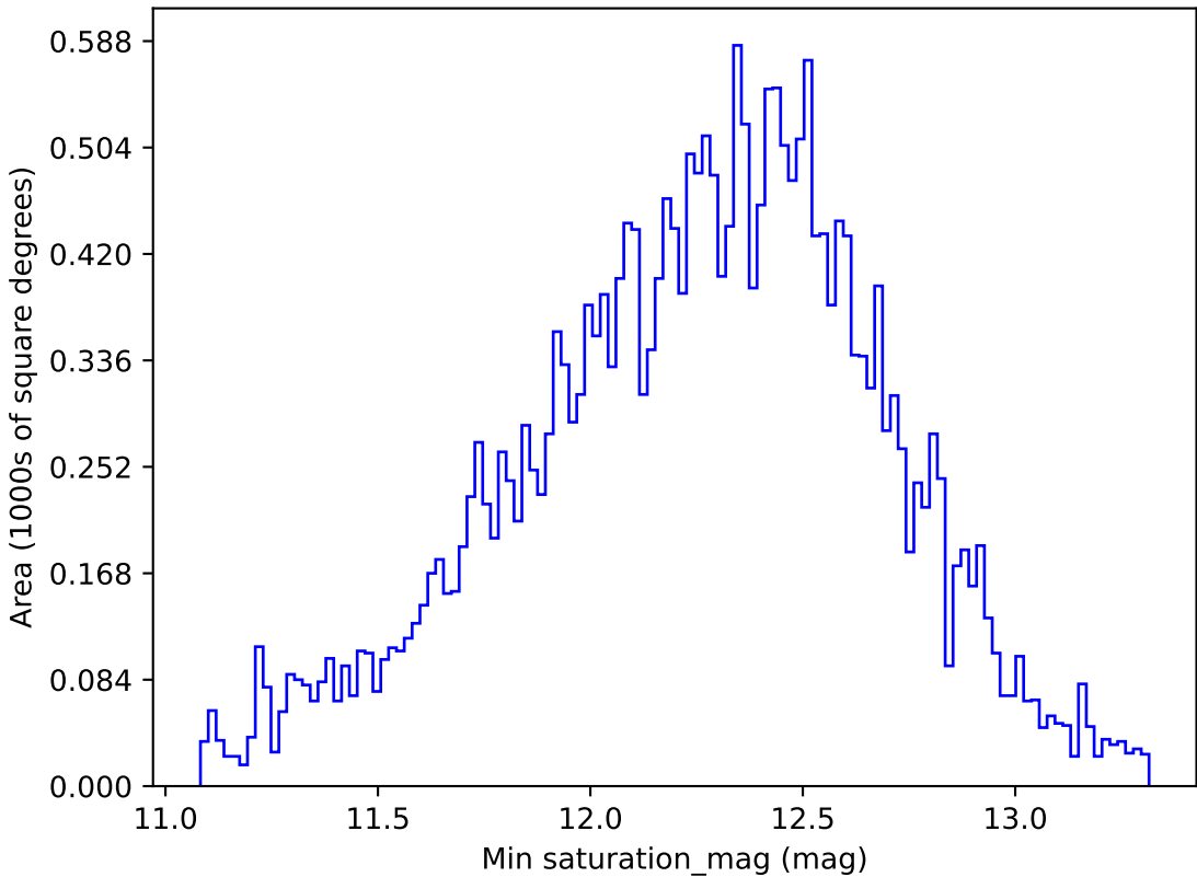
roll_pause_mjdp270_v3.4_10yrs All sky z band: Min saturation_mag
