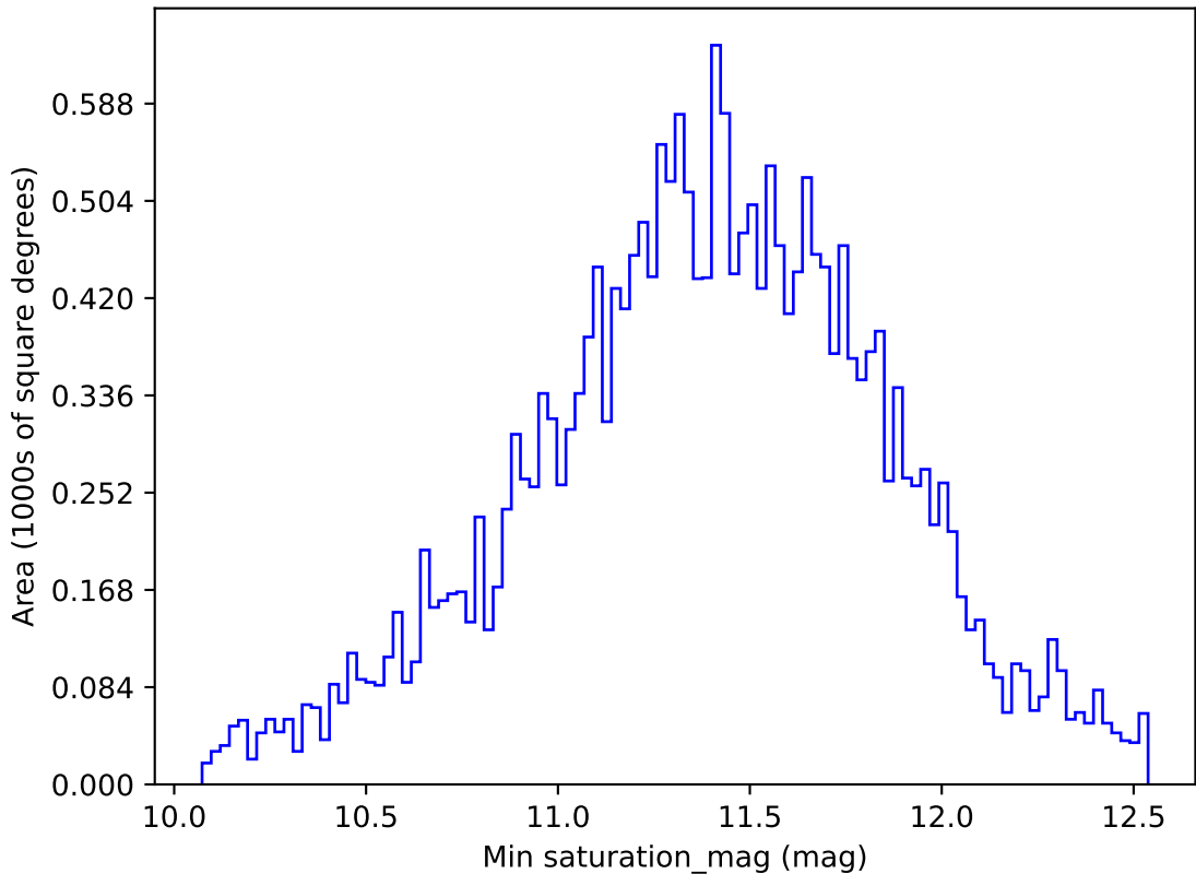
roll_pause_mjdp270_v3.4_10yrs All sky y band: Min saturation_mag
