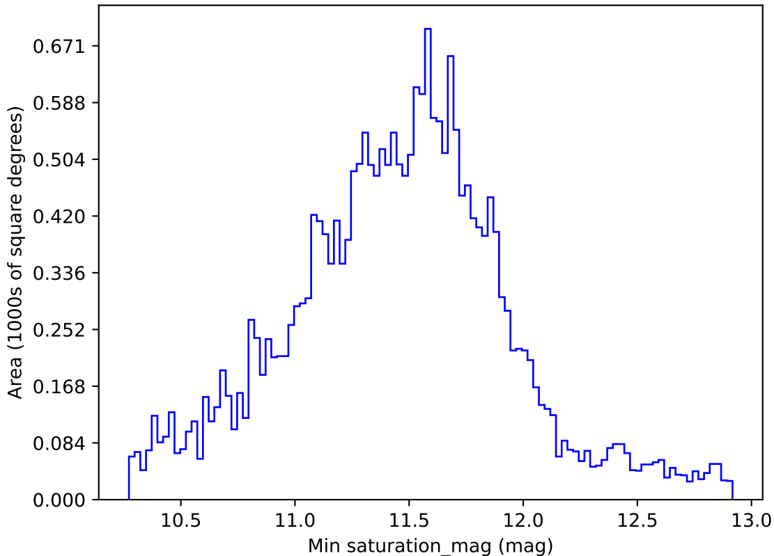
roll_pause_mjdp270_v3.4_10yrs All sky u band: Min saturation_mag
