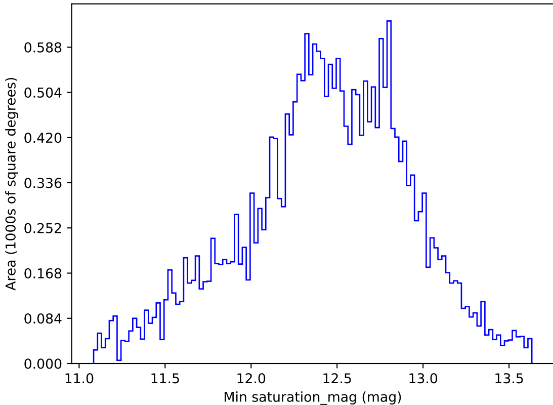
roll_pause_mjdp270_v3.4_10yrs All sky i band: Min saturation_mag
