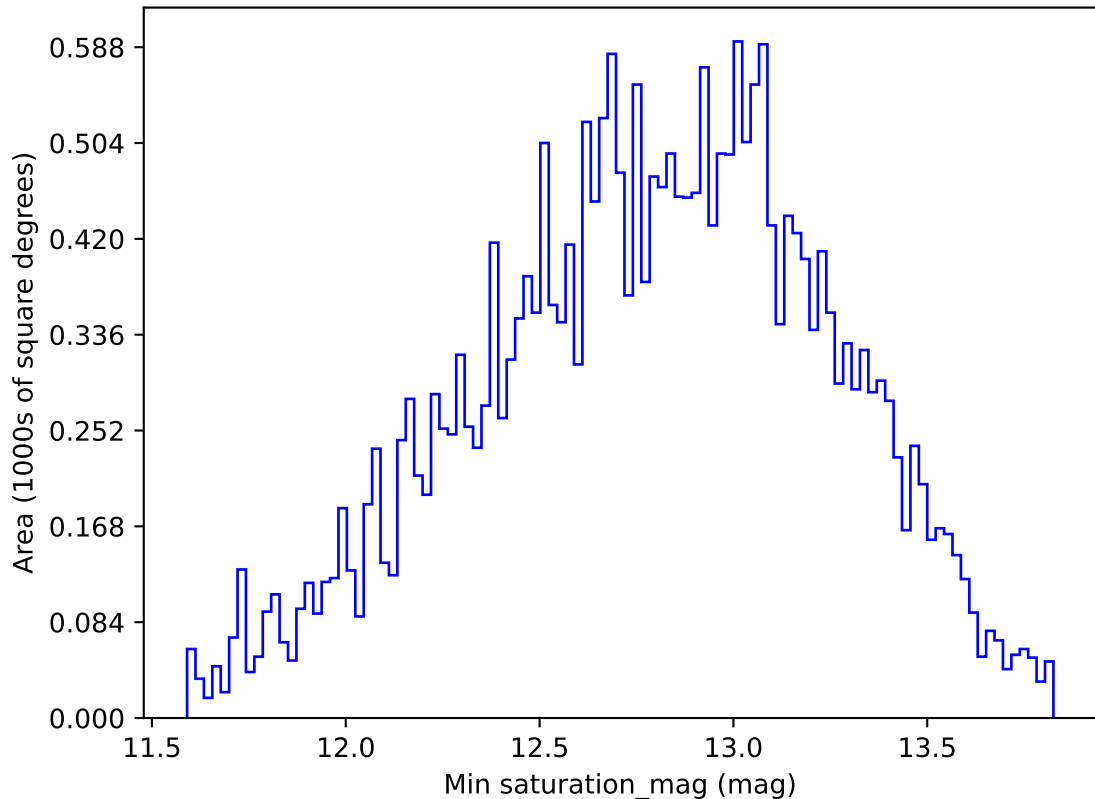
roll_pause_mjdp270_v3.4_10yrs All sky g band: Min saturation_mag
