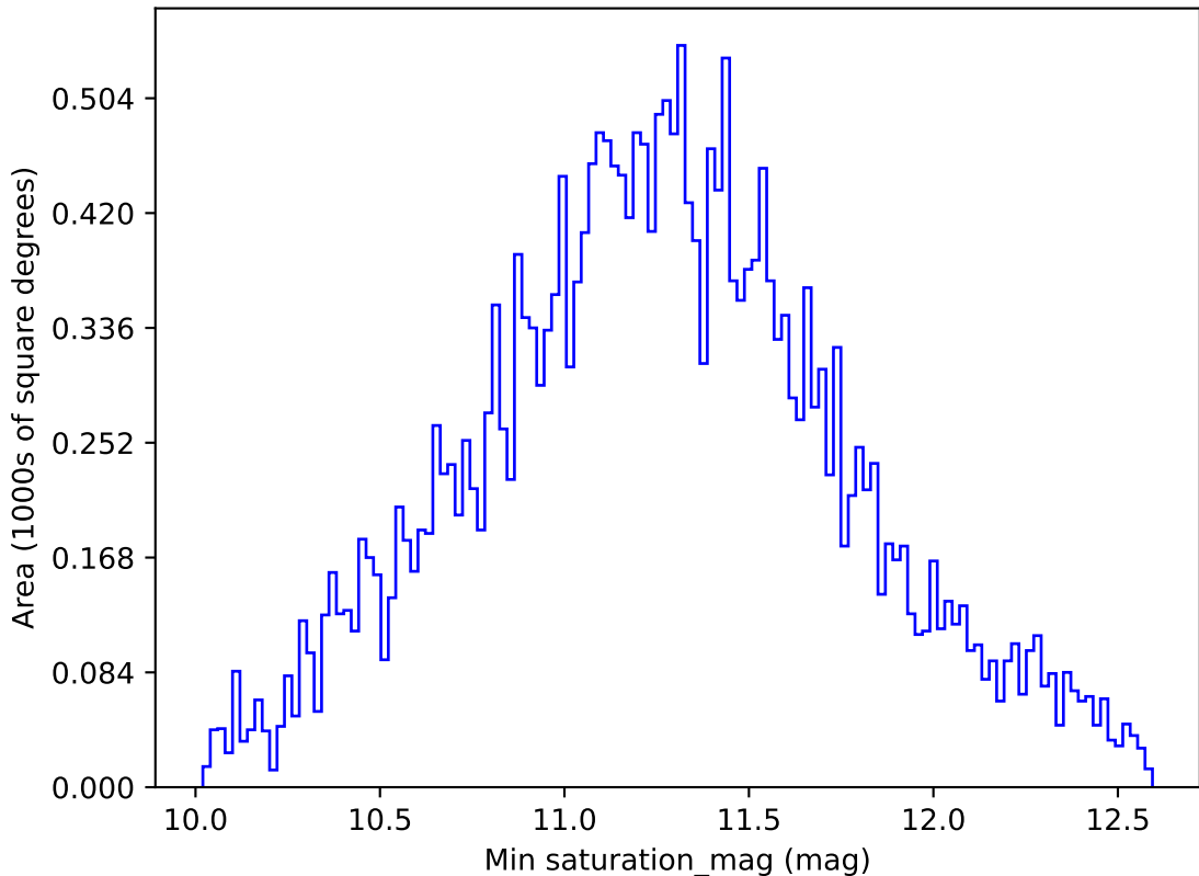
roll_pause_mjdp270_v3.4_10yrs All sky all bands: Min saturation_mag
