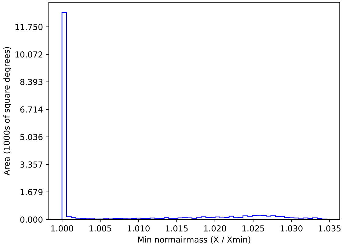
roll_pause_mjdp270_v3.4_10yrs WFD z band: Min normairmass
