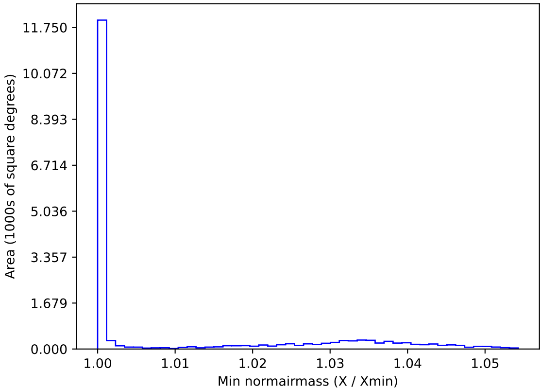
roll_pause_mjdp270_v3.4_10yrs WFD u band: Min normairmass
