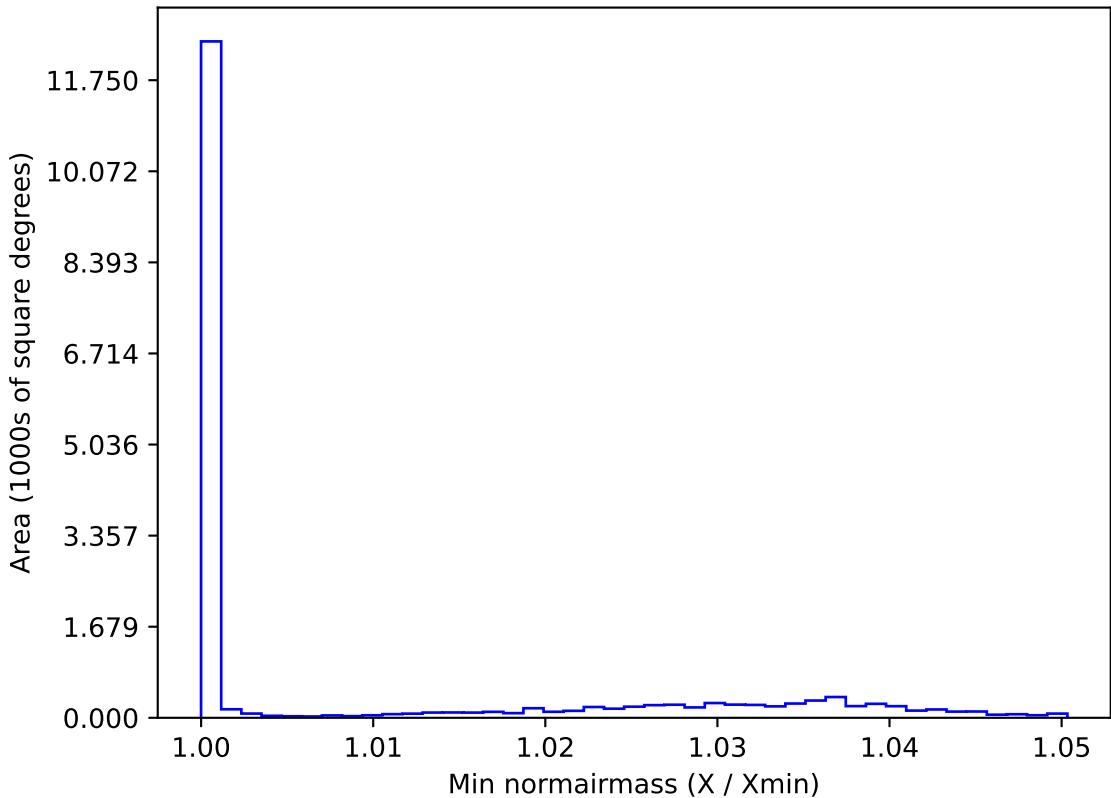
roll_pause_mjdp270_v3.4_10yrs WFD g band: Min normairmass
