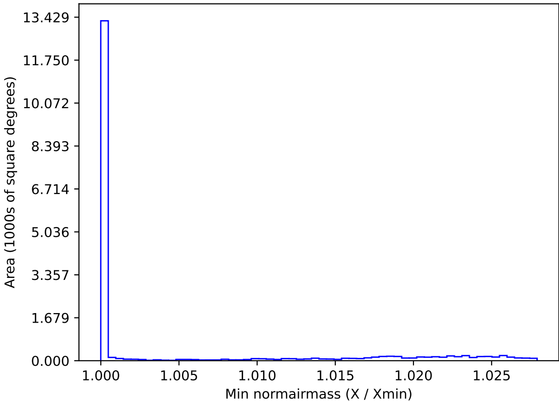
roll_pause_mjdp270_v3.4_10yrs WFD all bands: Min normairmass
