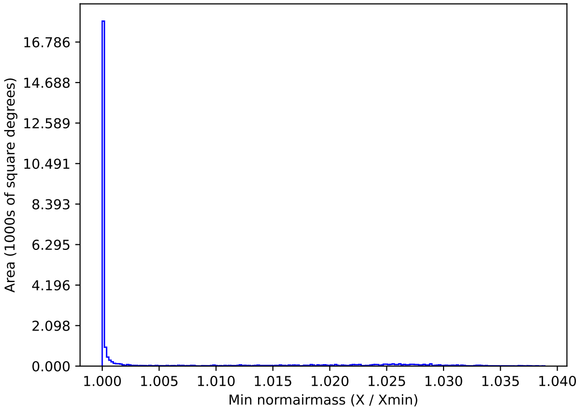
roll_pause_mjdp270_v3.4_10yrs All sky z band: Min normairmass
