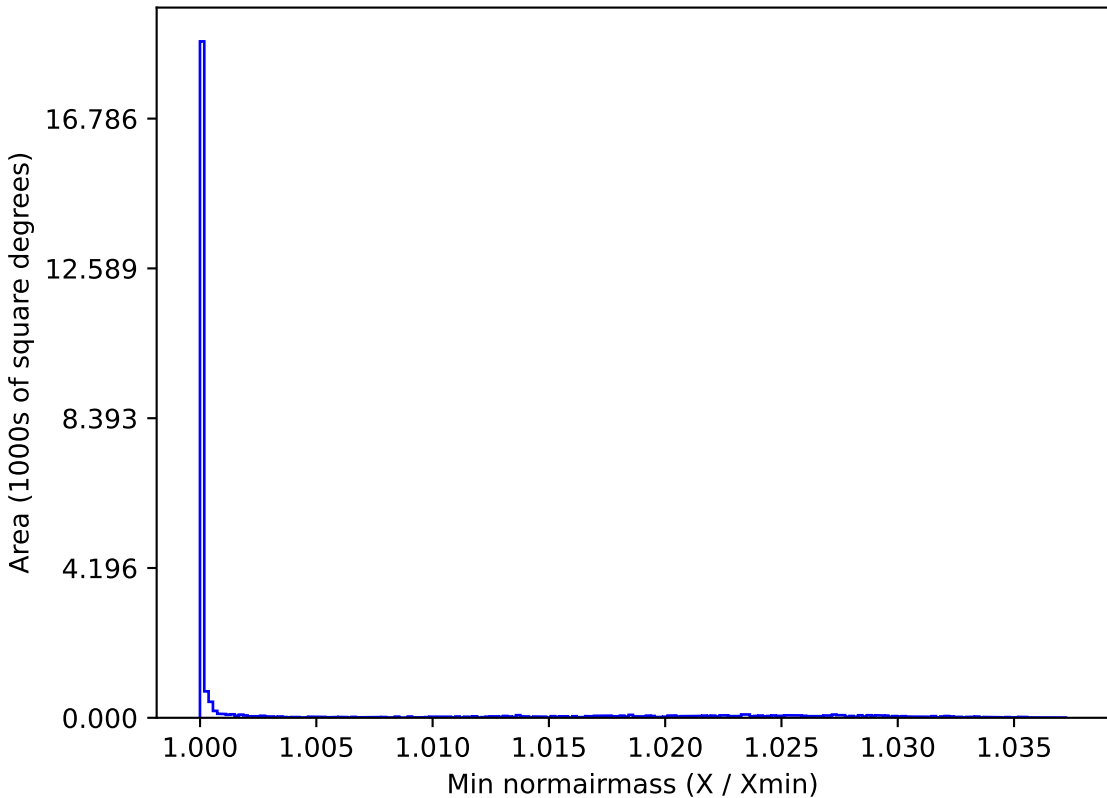
roll_pause_mjdp270_v3.4_10yrs All sky r band: Min normairmass
