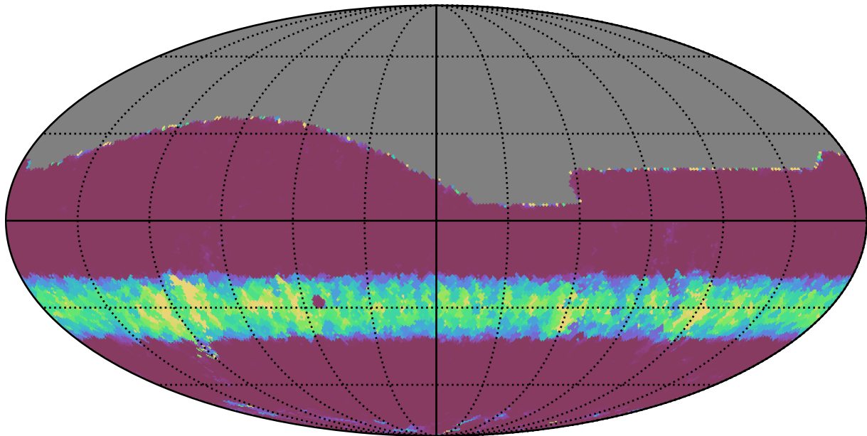
roll_pause_mjdp270_v3.4_10yrs All sky g band: Min normairmass
