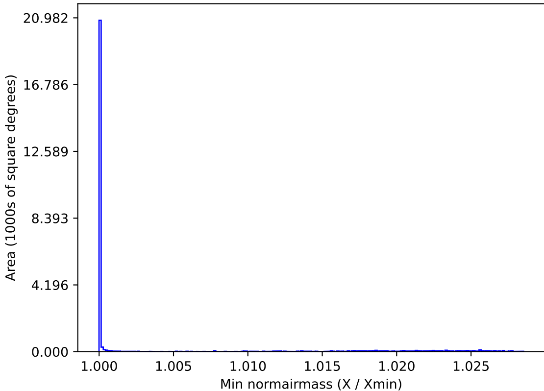
roll_pause_mjdp270_v3.4_10yrs All sky all bands: Min normairmass
