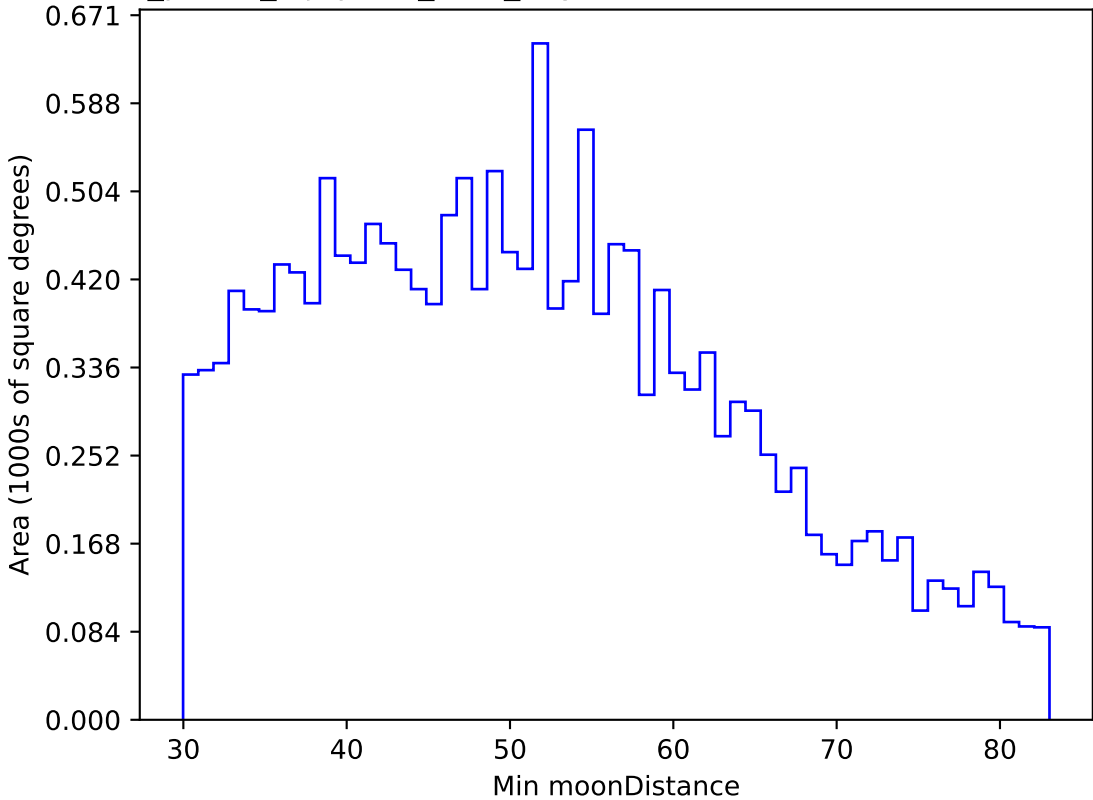
roll_pause_mjdp270_v3.4_10yrs WFD u band: Min moonDistance
