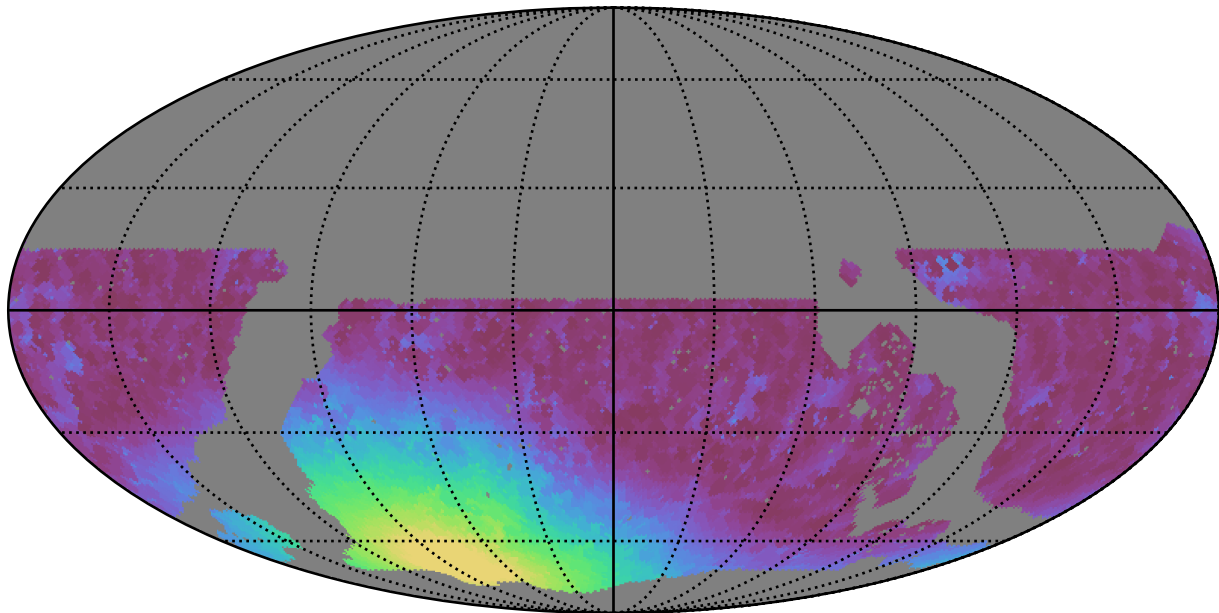
roll_pause_mjdp270_v3.4_10yrs WFD r band: Min moonDistance
