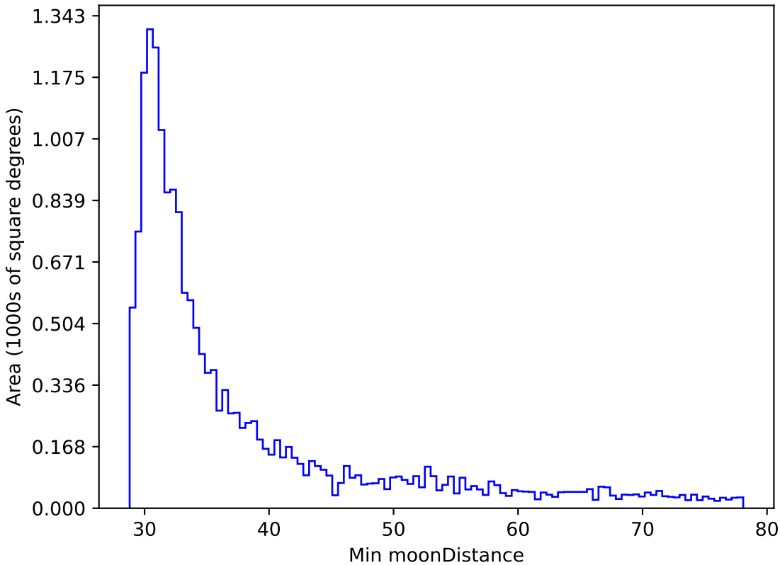
roll_pause_mjdp270_v3.4_10yrs WFD r band: Min moonDistance
