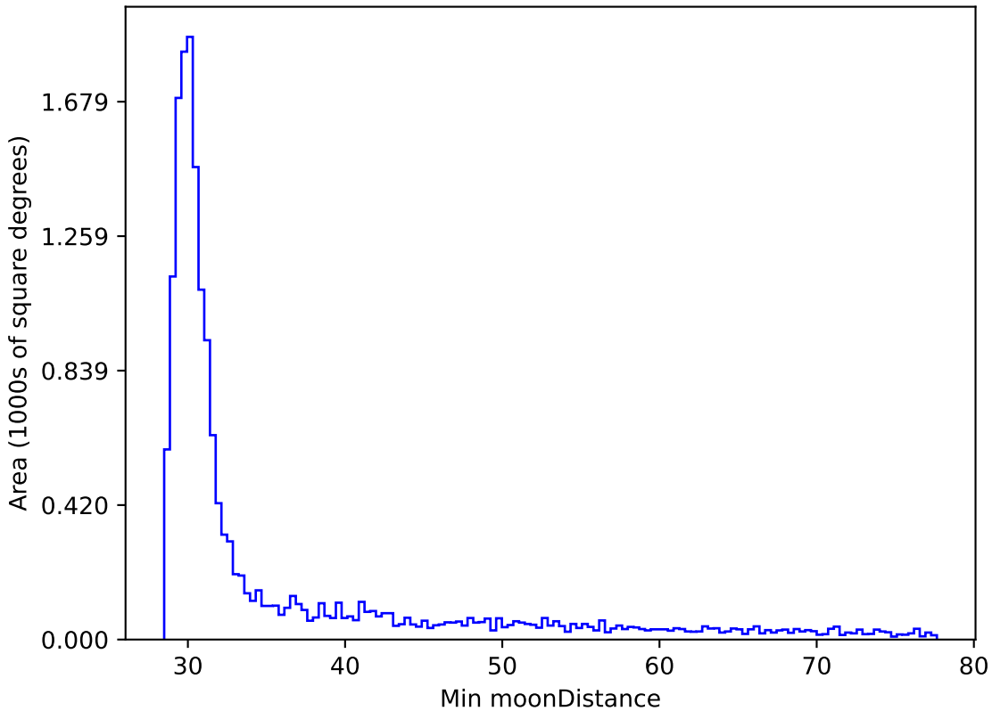
roll_pause_mjdp270_v3.4_10yrs WFD i band: Min moonDistance
