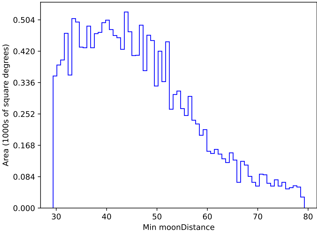
roll_pause_mjdp270_v3.4_10yrs WFD g band: Min moonDistance
