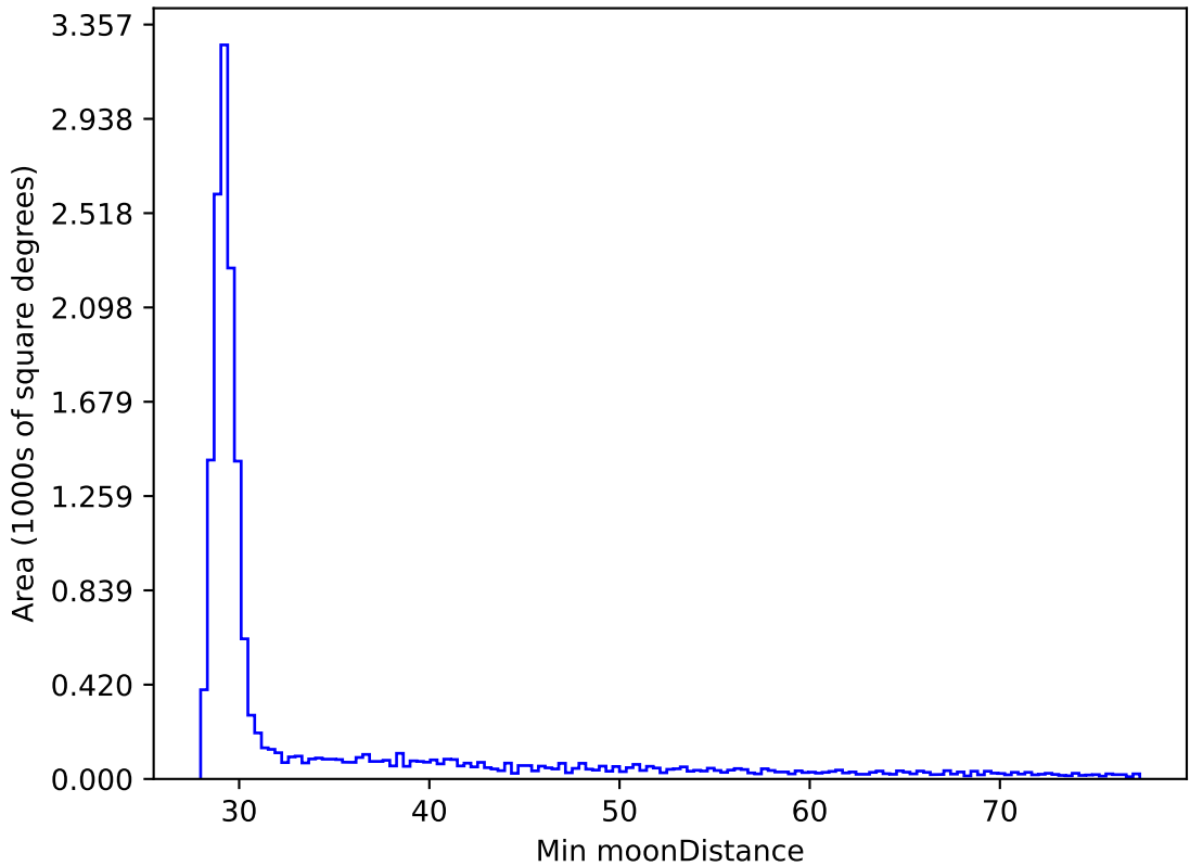
roll_pause_mjdp270_v3.4_10yrs WFD all bands: Min moonDistance
